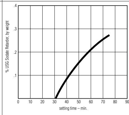
Fig. 8—Approximate retarding effect of USG Sodate Retarder on moulding, casting or pottery plasters.
