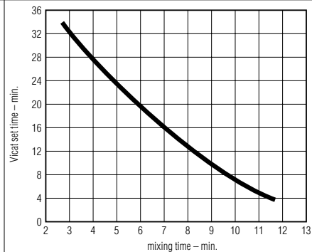
Fig. 4—Effect of mixing time on setting time.
